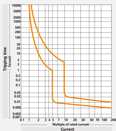
C curve
