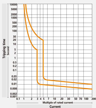
B curve
